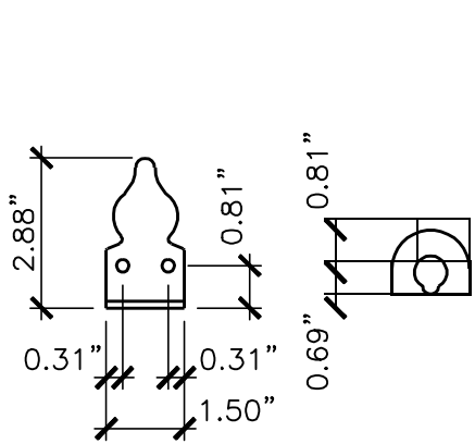
FRONT TOP FASTENER X2
